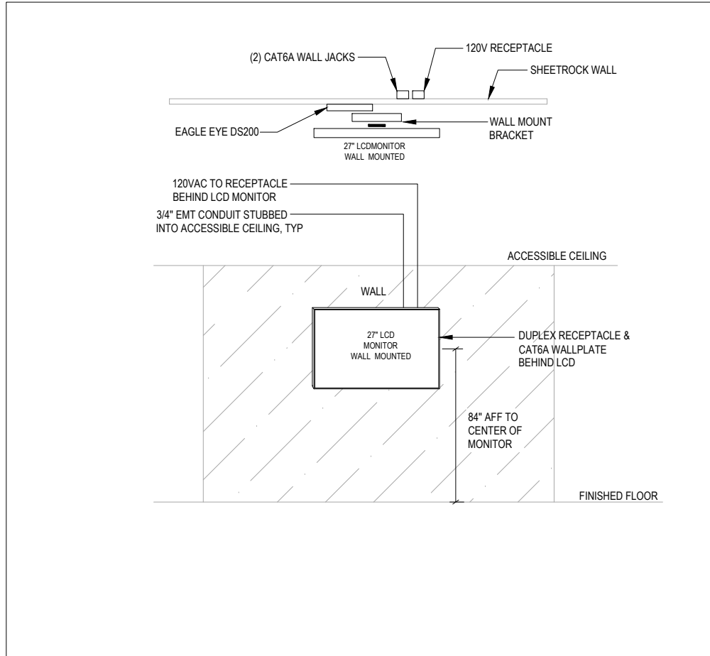
2 CAMERA VIEWING STATION SCALE: NONE
