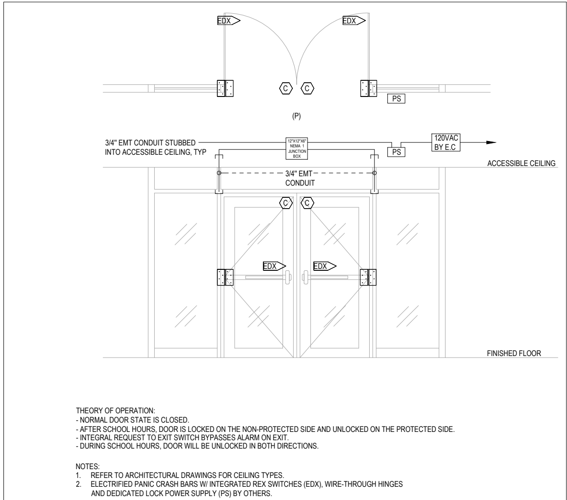
4 DOUBLE DOOR - EXIT DEVICE - UNLOCK ONLY SCALE: NONE
