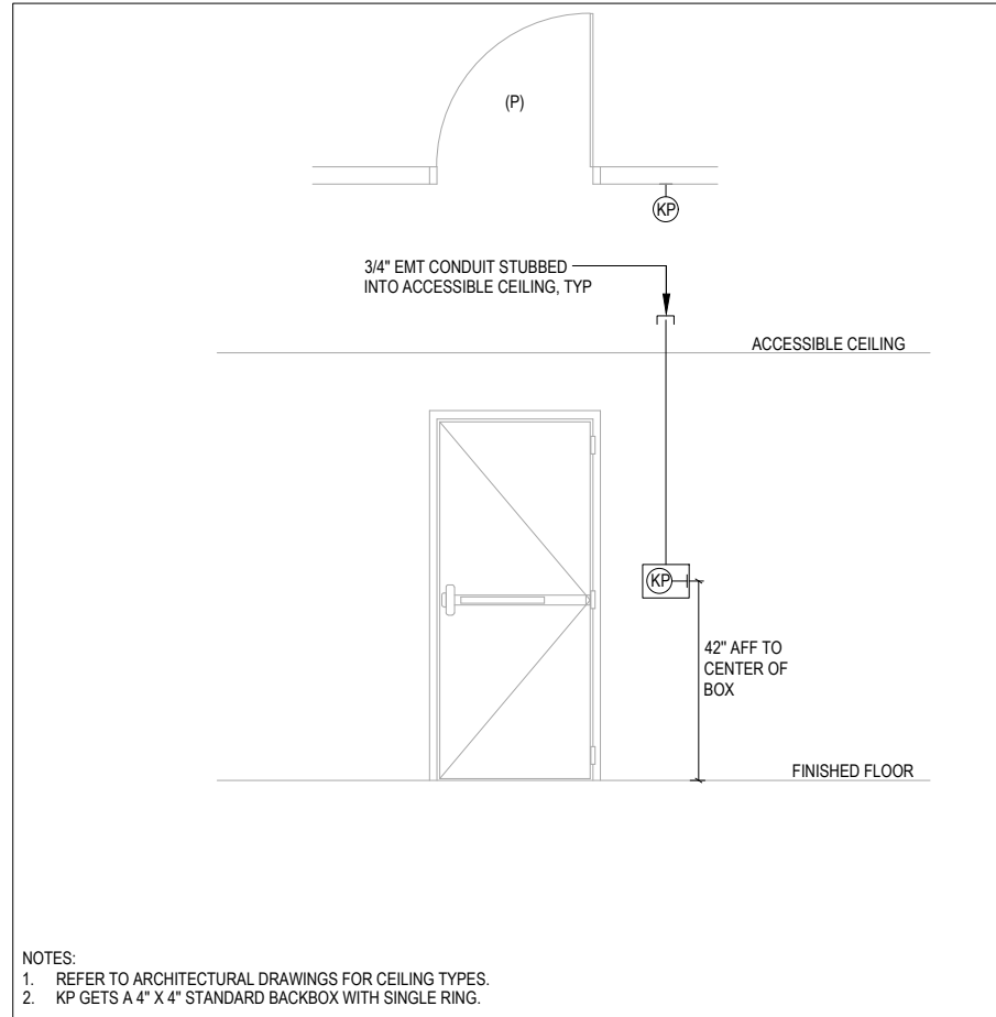
1 KEYPAD (ARMING/DISARMING) SCALE: NONE
